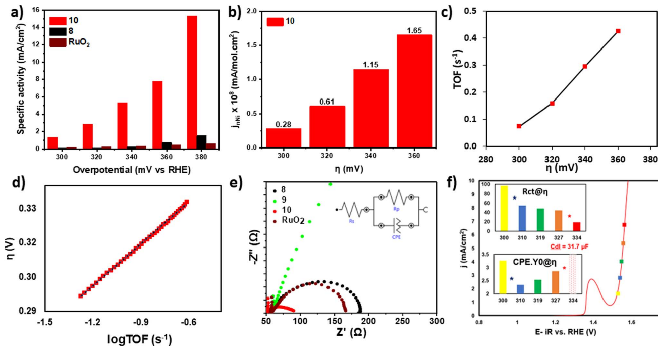
Fig. 3 (a) Tabulated values of specific activity j_{ECSA} of 10, 8 and RuO 2 across various overpotentials, (b) tabulated values of the intrinsic activity j_{Ni} of 10 across various overpotentials, (c) TOF as a function of \eta for electrocatalyst 10, (d) logarithmic TOF (log TOF) as a function of \eta for electrocatalyst 10, (e) Nyquist plots of 10, 9, 8 and RuO 2 (inset: applied Randles circuit fit) and (f) R_{ct} and CPE.Y0 across various overpotentials for 10. RDS changes are marked with stars.
