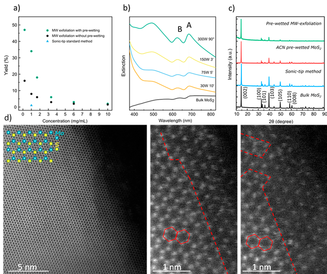
Figure 2. (a) Yield of the NMP-ACN exfoliated samples related to the initial concentration of bulk MoS 2 . (b) UV-vis spectra of various MoS 2 samples, exfoliated with different power-time conditions, compared to bulk MoS 2 (black). (c) Comparison of the XRD structure peaks disappearance of bulk MoS 2 (black), sonic-tip exfoliated MoS 2 (blue), ACN prewetted MoS 2 (red), and prewetted MW-exfoliated MoS 2 (green). (d) HAADF-STEM images with atomic resolution of MW exfoliated MoS 2 (2H phase). Inset, schematic illustration of the structure of MoS 2 . Red dashed line delimits the area where vacancy defects are located.
