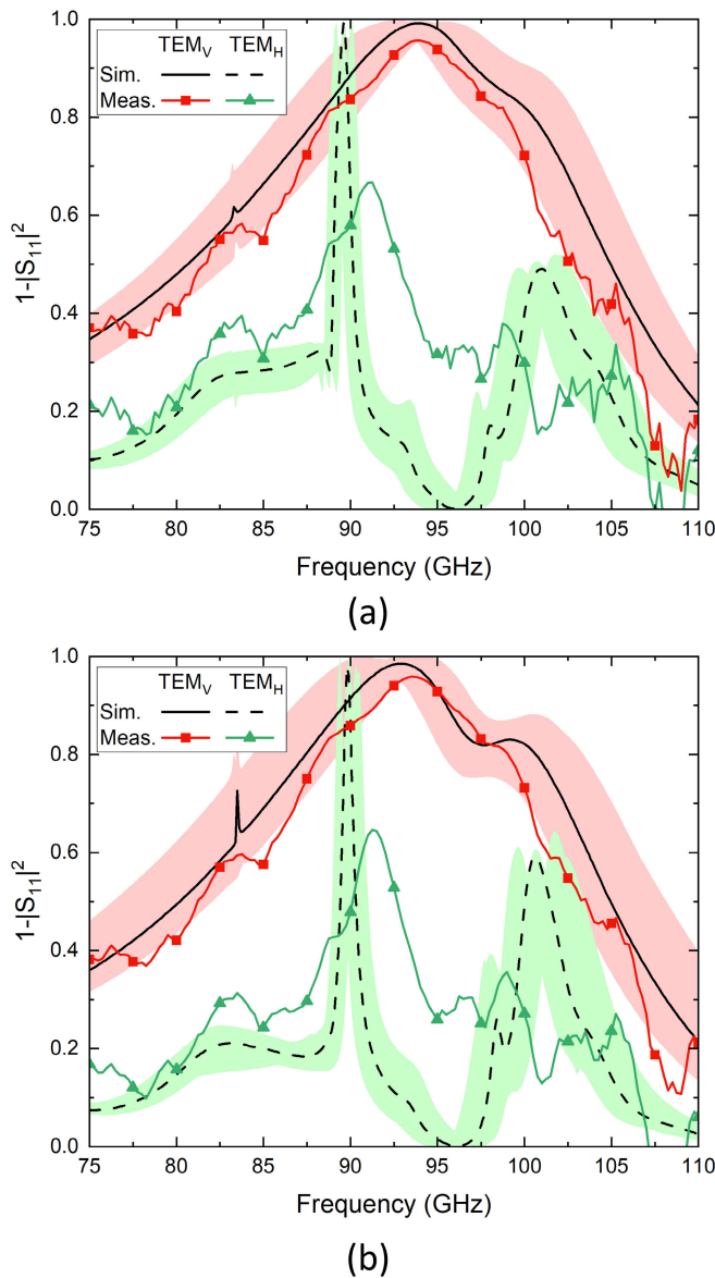
Fig. 8. Simulated and measured absorption at room temperature for the 39-nm aluminum LEKID ( R_s = 1.03 \Omega/\text{sq} ) on the silicon wafer. Linearly polarized incident wave for orthogonal polarizations. Sensitivity analysis (shaded areas). Silicon thickness 480 \pm 10 \mu\text{m} , air gap to the backshort 970 \pm 10 \mu\text{m} , and film thickness 39 \pm 3 \text{ nm} ( R_s = 1.16\text{--}0.99 \Omega/\text{sq} ). (a) LEKIDs in Fig. 1(a). (b) Sawtooth LEKIDs in Fig. 1(b).
