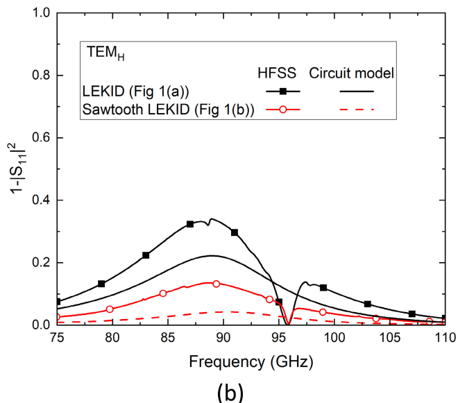
Fig. 3. LEKID absorption results for HFSS simulation and circuit model simulation without the interdigital capacitor. (a) Vertical E -field ( TEM_V ) referred to the position of the LEKIDs in Fig. 1. (b) Horizontal E -field ( TEM_H ) referred to the position of the LEKIDs in Fig. 1.
