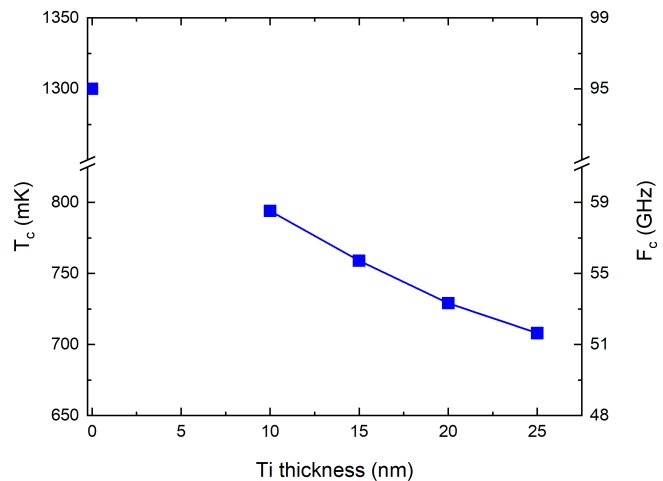
Fig. 4. Dependence of the critical temperature and cut-off frequency of the bilayer film with the titanium thickness over a 15-nm aluminum layer.
