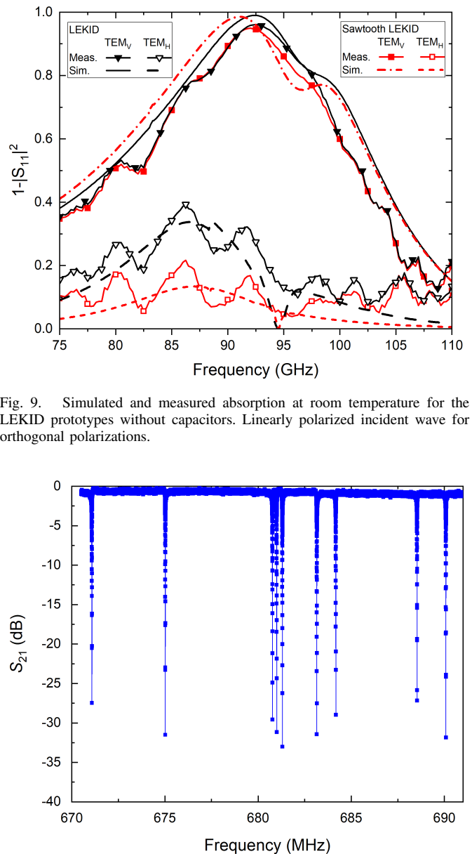
Fig. 10. Resonant frequencies for the fabricated 3 \times 3 LEKID array with the sawtooth strip, under dark conditions at T = 10 \text{ mK} , with an input power at the detector of P_{\text{in}} = -105 \text{ dBm} and a frequency step 1.025 kHz.
