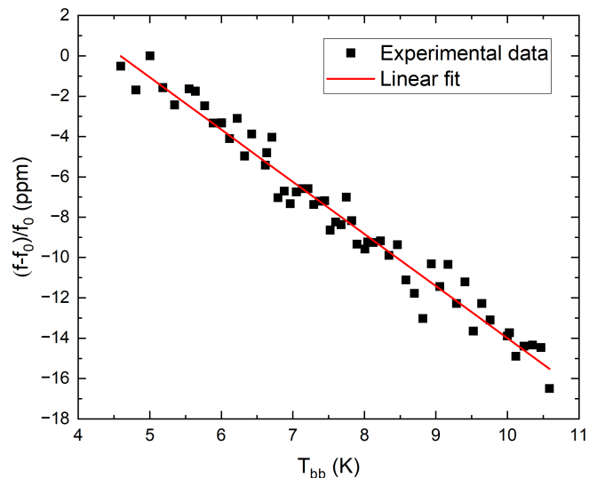
Fig. 13. Temperature dependence of the optical responsivity of the illuminated LEKID, with fitting parameters: r^2 = 0.96661 , \chi^2 = -0.98316 , and RMSE = 0.61627.
