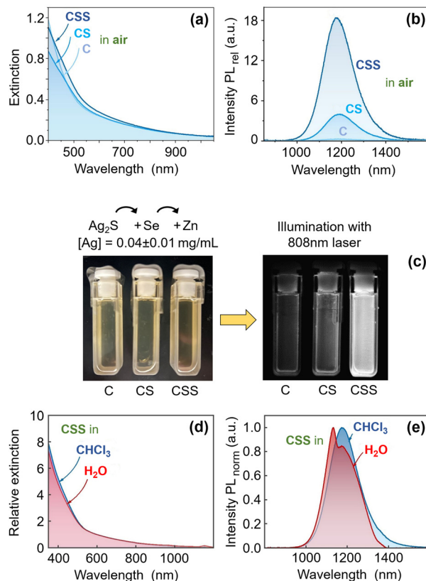
Fig. 2 (a) Extinction and (b) PL spectra of \text{Ag}_2\text{S} NCs cores, CS and CSS NCs, in air. (c) Optical images of the \text{Ag}_2\text{S} NCs cores, CS and CSS NCs solution samples without (left) and with (right) illumination with a NIR laser (808 nm). (d) Extinction and (e) PL responses of CSS NCs, dispersed in water and in chloroform.
