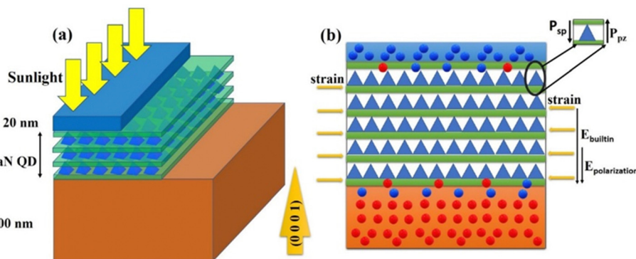
Fig. 1 (a) Epitaxial layer structure of IBSC based on In 0.5 Ga 0.5 N QDs embedded in a GaN matrix with 1 nm GaN interlayers. (b) Schematic diagram of polarization-induced charges, and the electric fields at the In 0.5 Ga 0.5 N/GaN interfaces. The inset shows the directions of spontaneous polarization ( P_{sp} ) and piezoelectric polarization ( P_{pz} ) at the interface.
