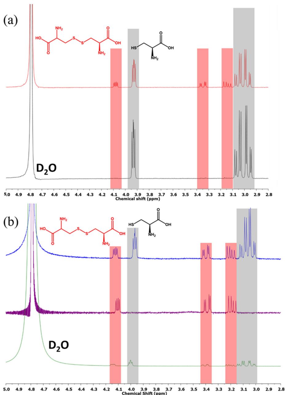
Fig. 2 (a) Representative 1 H-NMR spectra of 5 mM L-cysteine solution in D 2 O freshly prepared and after 24 h (black and red, respectively). The peaks highlighted in grey refer to L-cysteine and the peaks highlighted in red refer to cystine. (b) Representative 1 H-NMR spectra of 5 mM L-cysteine solution in D 2 O after 24 h of incubation with GO, rGO or GNPs (green, purple, and blue, respectively). The peaks highlighted in grey refer to L-cysteine and the peaks highlighted in red refer to cystine.
