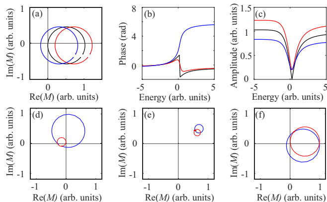
FIG. 7. (a) Complex representation of M(\epsilon) without background (black), with a positive background (red) and with a negative background (blue). (b) \arg[M(\epsilon)] and (c) |M(\epsilon)|^2 as a function of \epsilon for the three cases. [(d)–(f)] Channel resolved complex trajectory of the two-photon matrix element in the vicinity of SB16 calculated with RPAE with the final state (d) \epsilon p^1S , (e) \epsilon p^1D , and (f) \epsilon f^1D . The red (blue) lines indicate the results without (with) final state interactions. The amplitudes of the complex trajectories in (d)–(f) have been normalized to the respective maximum radius in each panel.
