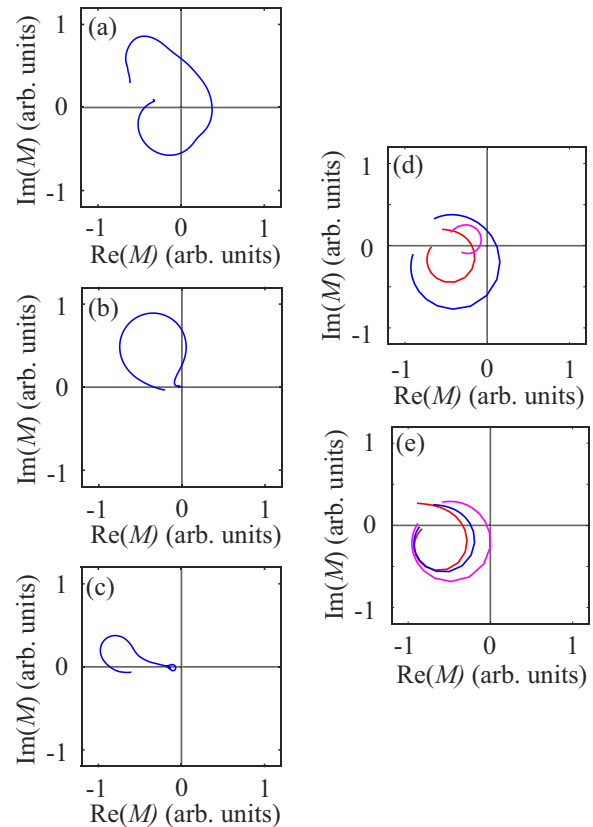
FIG. 8. [(a)–(c)] Channel resolved complex trajectory of the two-photon matrix element in the vicinity of SB16 calculated with NEWSTOCK with the final state (a) {}^2P_{1/2} \ \epsilon p_{1/2} \ ^1S , (b) {}^2P_{1/2} \ \epsilon p_{3/2} \ ^1D , and (c) {}^2P_{1/2} \ \epsilon f_{5/2} \ ^1D . [(d)–(e)] Complex trajectory of the coherent superposition of the \epsilon p \ ^1S and \epsilon p \ ^1D two-photon matrix elements in the lower sideband, calculated with XCHEM. In (d), the probe pulse duration is 12 fs and the probe photon energy is 1.27 (red), 1.55 (blue), and 1.65 eV (magenta). In (e), the probe photon energy is 1.27 eV and the probe pulse duration is 8 (red), 12 (blue), and 22 fs (magenta). The amplitudes of the complex trajectories have been normalized to the respective maximum radius in each panel.
