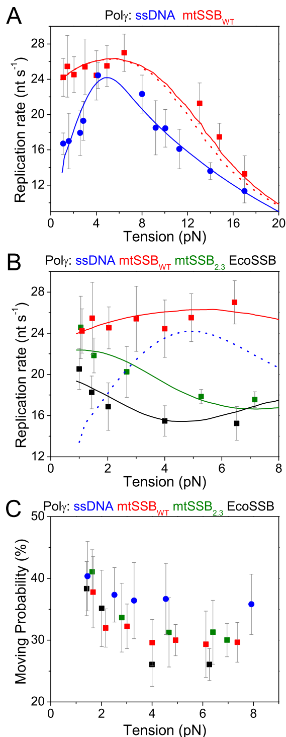
Figure 2. Effect of homologous and non-homologous SSBs on Poly replication kinetics. (A) Change of V_{\max} (nt s -1 ) with tension in SSB-free (blue symbols, N = 100 ) and mtSSB WT -covered (red symbols, N = 109 ) ssDNA. Lines represent best fit to data with Equation (1) (solid blue line), Equation (2) (solid red line) and Equation (4) (dotted red line). (B) Tension dependence of V_{\max} (nt s -1 ) in ssDNA covered either with mtSSB WT (red symbols), mtSSB 2.3 (green symbols, N = 57 ) or EcoSSB (black symbols, N = 30 ). Solid lines represent best fit of the data with Equation (4). For reference, dotted blue line shows fit to V_{\max} in SSB-free ssDNA (as shown in A). (C) Moving probability (average velocity/ V_{\max} ) of Poly on ssDNA (blue) and on ssDNA covered with mtSSB WT (red), mtSSB 2.3 (green) and EcoSSB (black). For all figures, error bars show standard errors.
