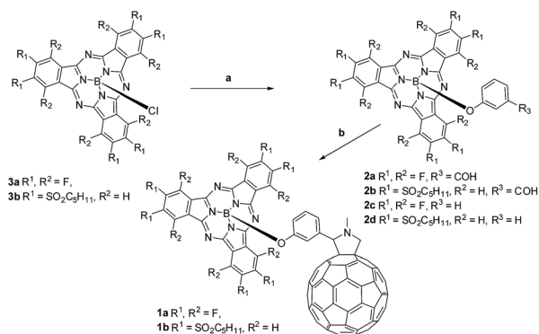
Scheme 1 Synthesis of SubPc–C 60 conjugates 1a,b . Conditions: (a) AgOTf, 3-hydroxybenzaldehyde/phenol, toluene; (b) N -methylglycine, C 60 , toluene, reflux.
